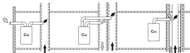
fig. 25 - Examples of connection to flues (→ = Air / → = Fumes)
