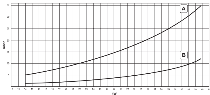
fig. 37 - Pressure - power diagram DIVAtop MICRO F 37
