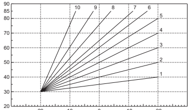
fig. 14 - Compensation curves
