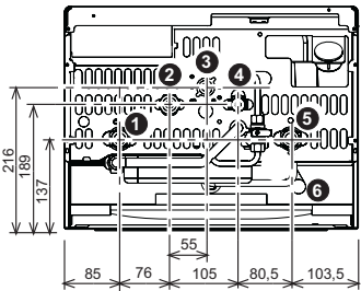
fig. 17 - Raccordements hydrauliques
