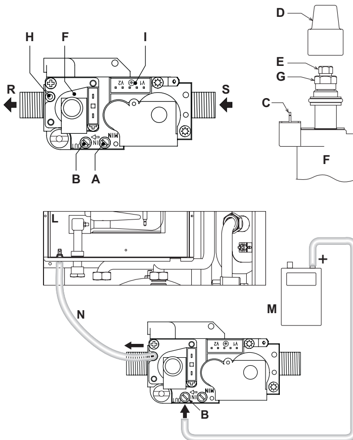
fig. 27 - Gas valve
