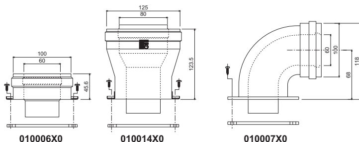
fig. 22 - Starting accessories for coaxial ducts
