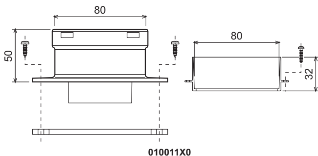
fig. 24 - Starting accessory for separate ducts
