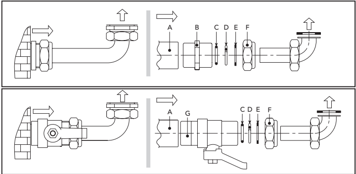
fig. 18 - Connection kit
