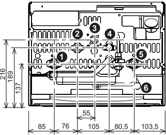
fig. 17 - Plumbing connections
