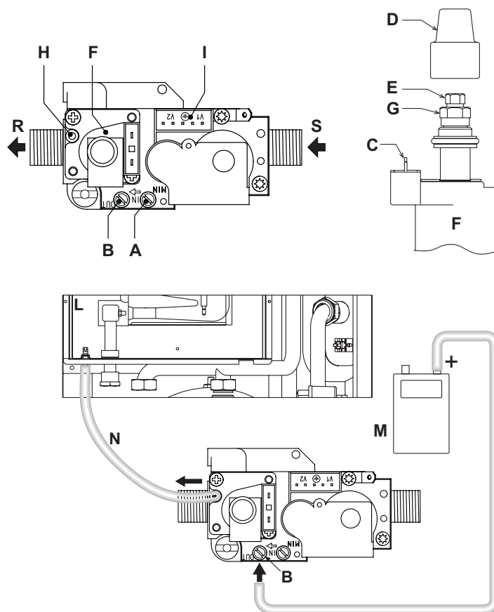
fig. 27 - Valvola gas
