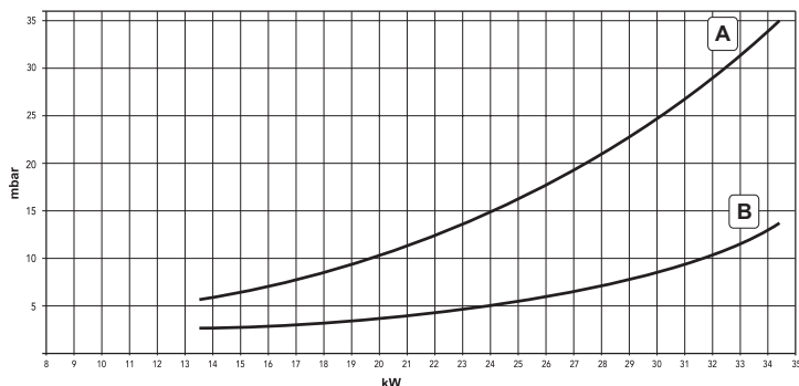
fig. 35 - Pressure/power diagram DIVAtop MICRO F 32
